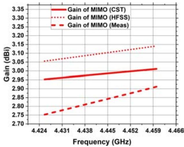
Figure 22. The suggested MIMO antenna's gain.
