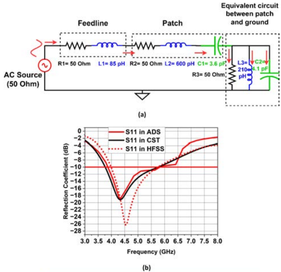
Figure 11. (a) Corresponding circuit design of the single antenna element, (b) Reflection coefficient simulated in CST vs HFSS vs ADS.
