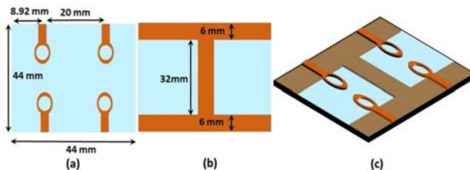
Figure 17. A 2 \times 2 MIMO antenna including vertical strip (a) front view, (b) back view, (c) exploded view.
