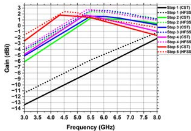
Figure 12. Gain of the single antenna element at every stage of the development.
