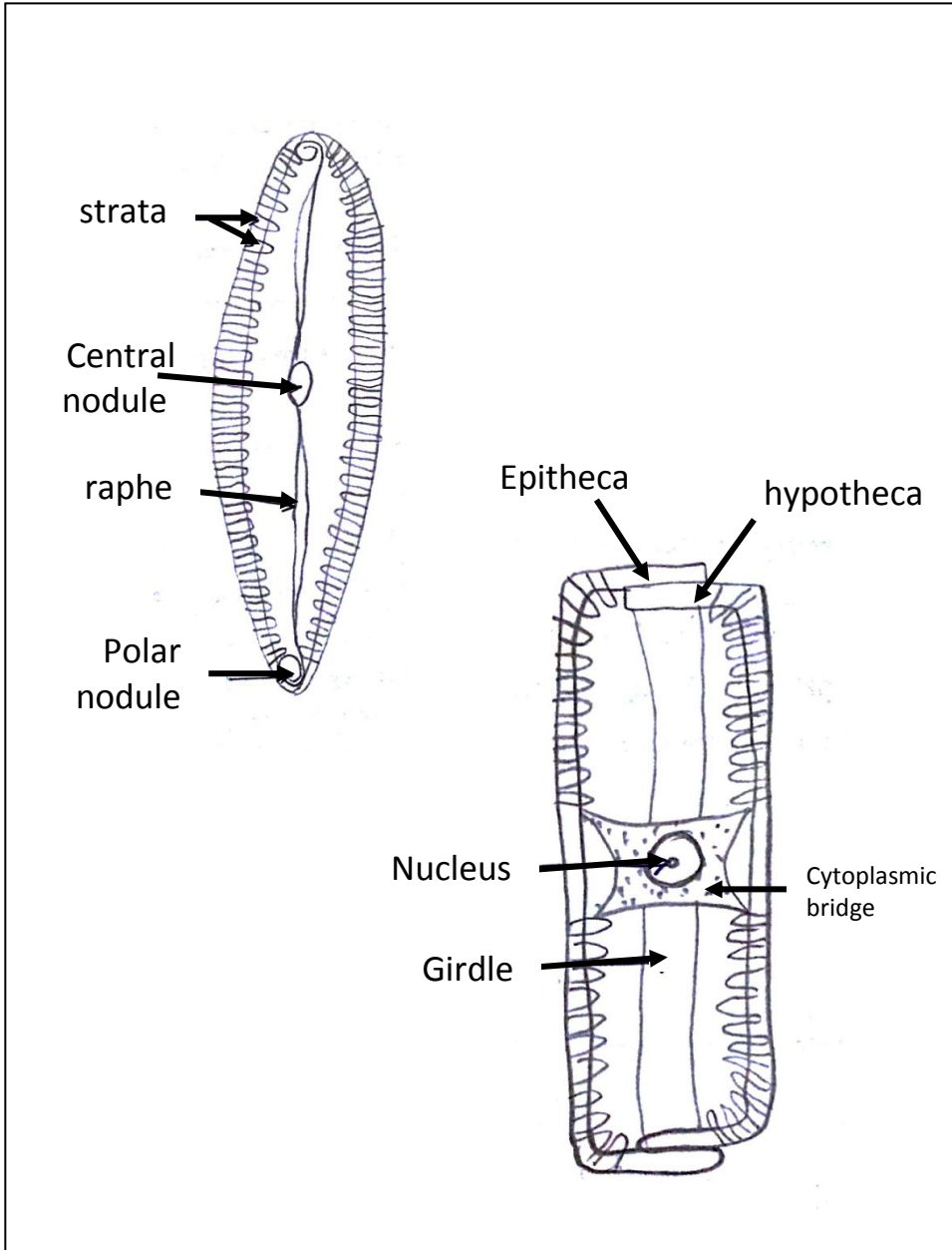
Diatoms
