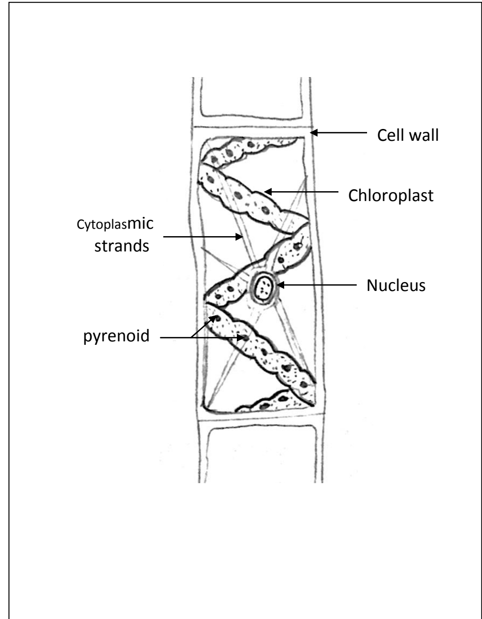
G : Spirogyra
