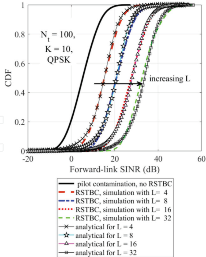
Figure 9. CDF simulation and analytical results' comparisons of SINR for multi-cell massive MU-MIMO system with N_t = 100 , K = 10 , QPSK, pilot reuse factor = 3/7, RSTBC with L = 4, 8, 16, 32 , and 25% loss rate. Analytical curves are plotted using Eq. (21) in [43].
