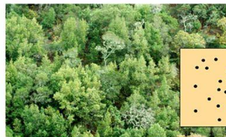
(c) Random
