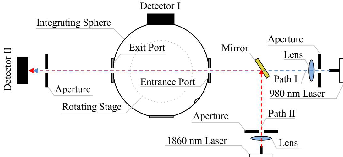
Figure 3.1: A schematic top view of the single integrating sphere system setup. The mirror is mounted on a rotating stage to switch between path I and path II. When the mirror is rotated to 334^\circ the 980 nm CW laser path (Path I) is open. When using the 1860 nm pulsed laser system (Path II) mirror should be rotated back 334^\circ to allow the mirror to reflect the laser beam inside the integrating sphere. The integrating sphere is mounted on a rotating stage as well. The rotating stage gives the ability to the integrating sphere to switch between diffuse transmittance and diffuse reflectance modes.
