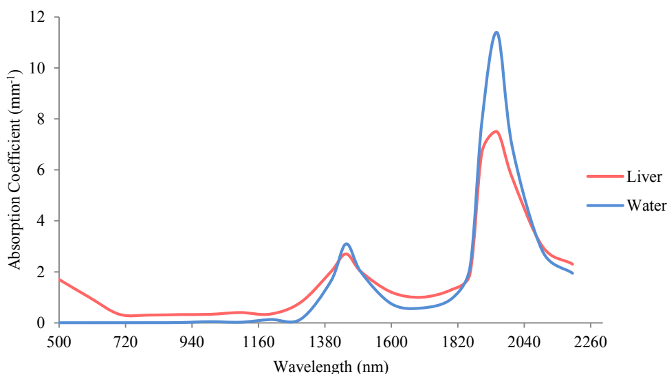
Figure 5.1: The absorption coefficient of a rat liver (red) and water (blue) in a wide range of wavelengths between 500 and 2200 nm. There are two distinguished peaks in the IR region at 1420 and 1940 nm. The absorption coefficient of rat liver was adapted from (Parsa, et al., 1989). The absorption coefficient of water was adapted from (Hale & Querry 1973).
