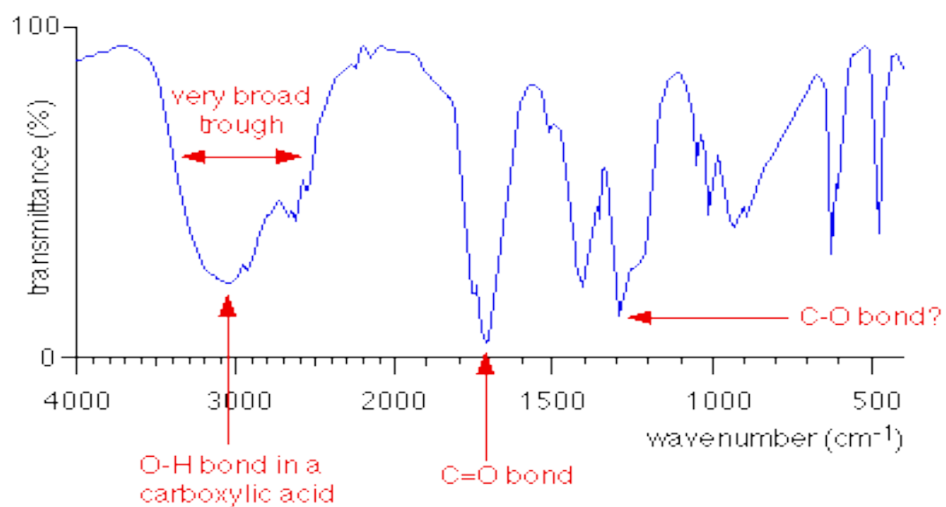
infra-red spectrum of ethanoic acid, \text{CH}_3\text{COOH}
