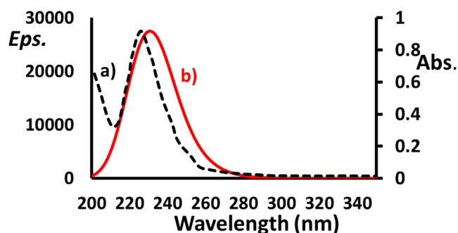
Fig. 8. UV-Visible and TD-DFT spectra of BDMDO in MeOH.
