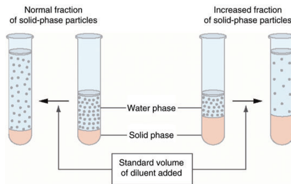
FIGURE 5: Pseudo-hyponatraemia. Normally, serum contains 7% solids by volume. In order to reduce the volume of blood needed for analysis, serum is frequently diluted before the actual measurement is obtained. The same volume of diluent is always used; the degree of dilution is estimated under the assumption that the serum contains 7% solid-phase particles. When the fraction of solid-phase particles is increased, the same amount of diluent results in a greater dilution, unbeknownst to the laboratory personnel (right side of figure). Consequently, the calculation of an ion level with the use of a degree of dilution that is based on the incorrect fraction of solid-phase particles will lead to an underestimate. Reproduced with permission from Massachusetts Medical Society Copyright © 2003 Turchin A, Seifter JL & Seely EW. Clinical problem-solving. Mind the gap. New England Journal of Medicine 2003 349 1465–1469.
