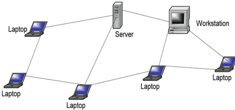
Fig. 13.6 Mesh network
