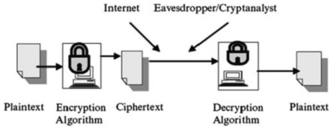
Fig. 13.8 Symmetric encryption
