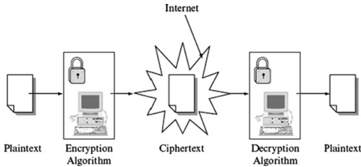
Fig. 5.1 Symmetric encryption
