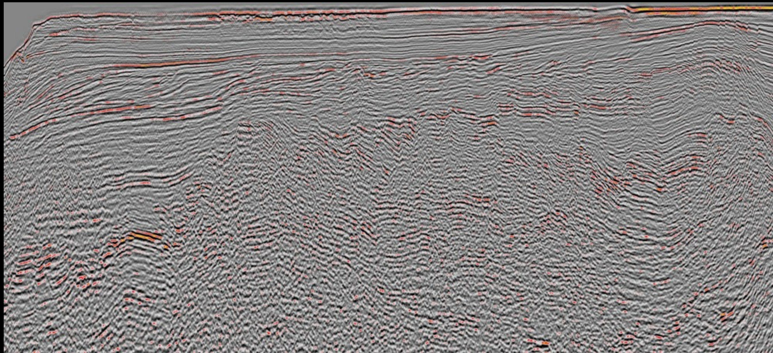
Outer Shelf Domino-Style Extensional Faults
