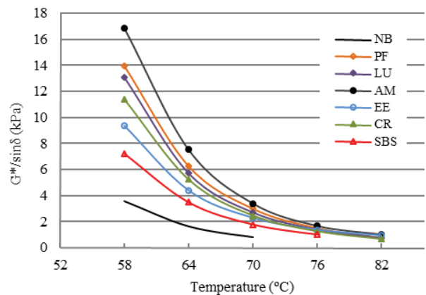
Fig. 4 G^*/\sin\delta vs. temperature for un-aged binders
