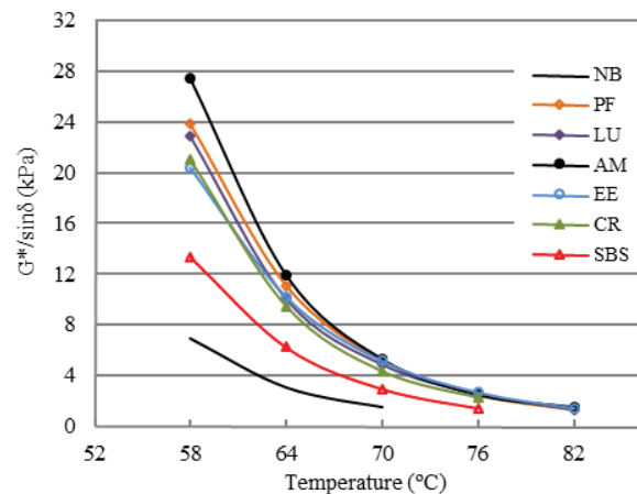
Fig. 5 G^*/\sin\delta vs. temperature for RTFO aged binders
