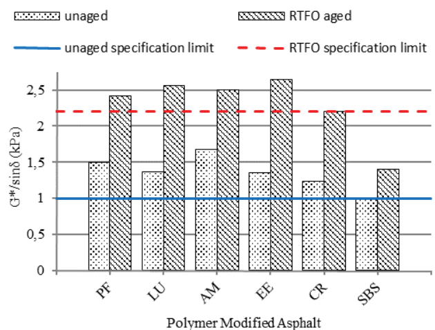
Fig. 6 G^*/\sin\delta at 76 °C for un-aged and RTFO aged polymer modified asphalt binders
