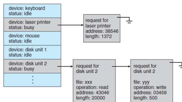
Figure 13.9 Device-status table.
