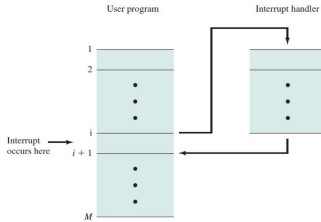
Figure 1.6 Transfer of Control via Interrupts
