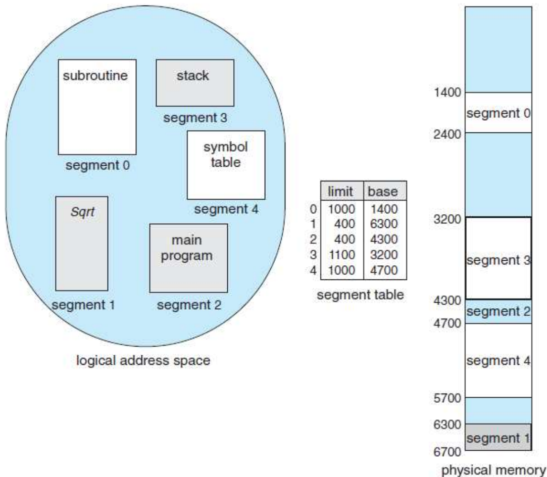
Figure 8.9 Example of segmentation.
