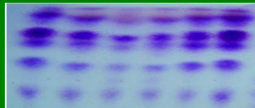
Chemistry
