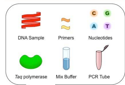
PCR Components
