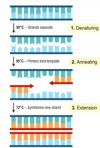
PCR Process (ONE Cycle)
