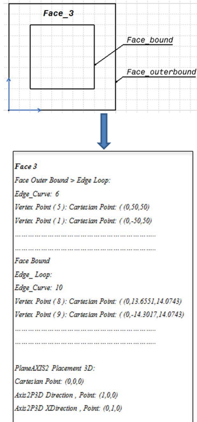
Fig. 3 Face_outerbound and Face_bound loops
