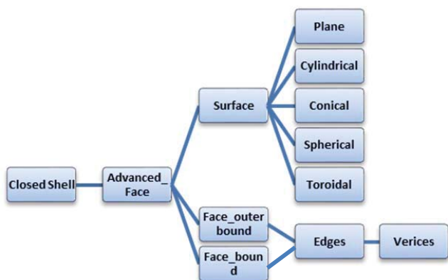
Fig. 1 STEP Data Structure
