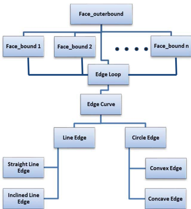
Fig. 4 Face-Loop-Edge Hierarchy
