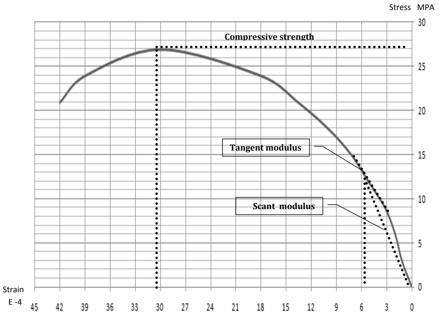
stress - strain curve
