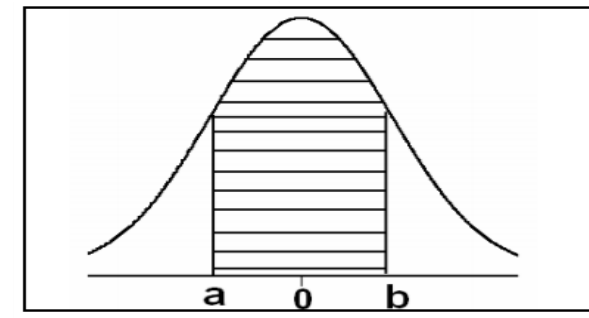
P(a \leq Z \leq b) = P(Z \leq b) - P(Z \leq a)
