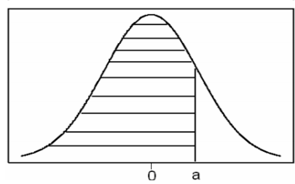
P(Z \leq a) = \text{From the table}
