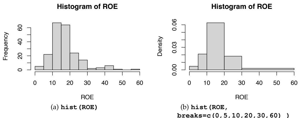
Figure 1.18. Histograms
