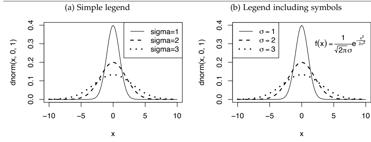
Figure 1.9. Using legends
