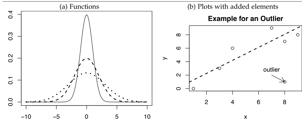
Figure 1.7. Overlaid plots
