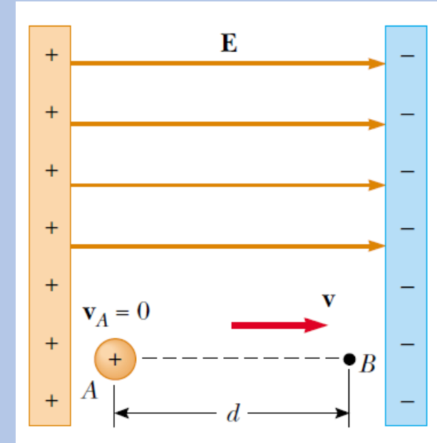
A proton accelerates from A to B in the direction of the electric field.
