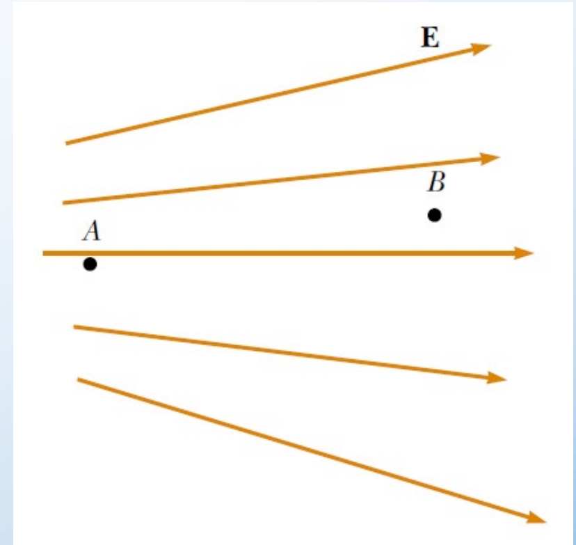
Two points in an electric field.
