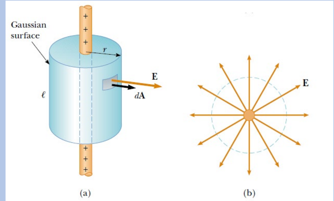
(a) An infinite line of charge surrounded by a cylindrical gaussian surface concentric with the line. (b) An end view shows that the electric field at the cylindrical surface is constant in magnitude and perpendicular to the surface.
