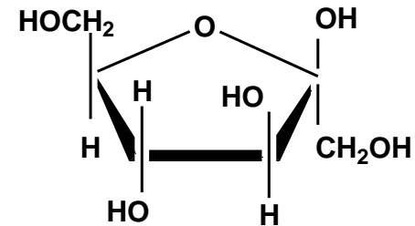
D-Fructose Fruit sugar
