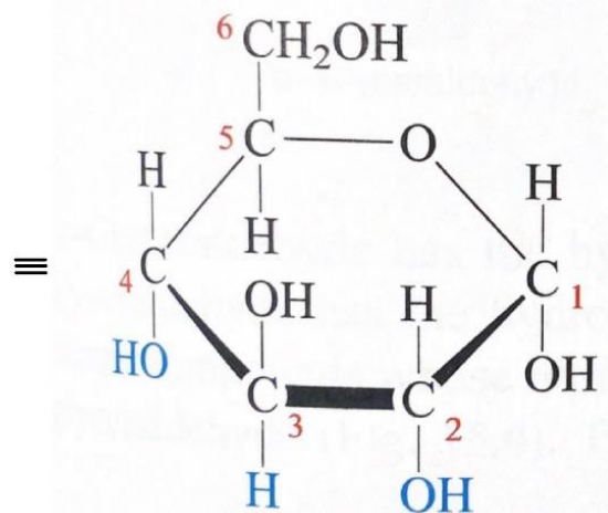
Haworth formula
