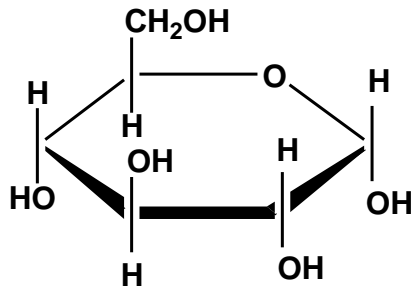
D-Glucose Blood sugar
