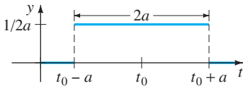
(a) graph of \delta_a(t - t_0)
