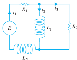
FIGURE 8.3.2 Network in Problem 33
