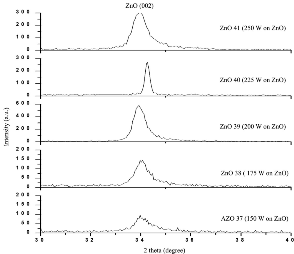
Fig. 2. XRD spectra of AlN: ZnO thin films at a different of RF power on Si substrates.
