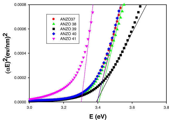
Fig. 5. (\alpha E)^2 versus E of AIN: ZnO films on glass at various RF powers on glass substrates.
