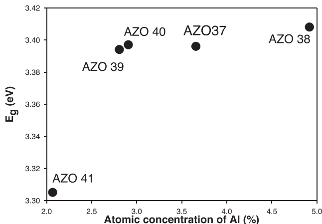
Fig. 6. Direct energy gap ( E_g ) versus Al at % concentration of AIN: ZnO thin films at different RF powers on glass substrates.
