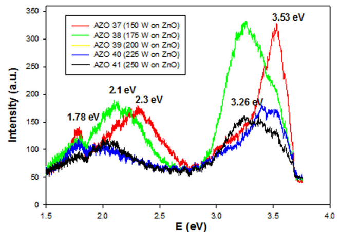
Fig. 7. The PL spectra of AIN: ZnO thin films at different RF powers on Si substrates.
