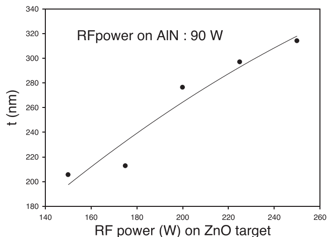
Fig. 1. Thickness of AlN: ZnO thin films as a function of RF power on Si substrates.
