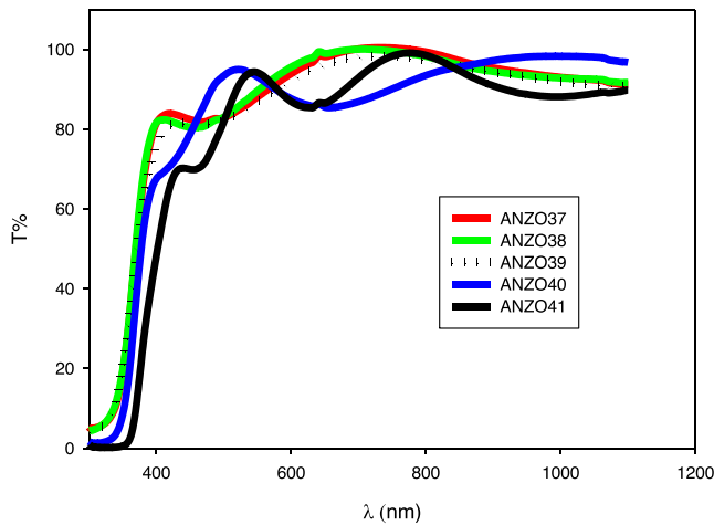
Fig. 4. AIN: ZnO Transmittance spectra of the prepared thin films on glass substrates at different RF powers.
