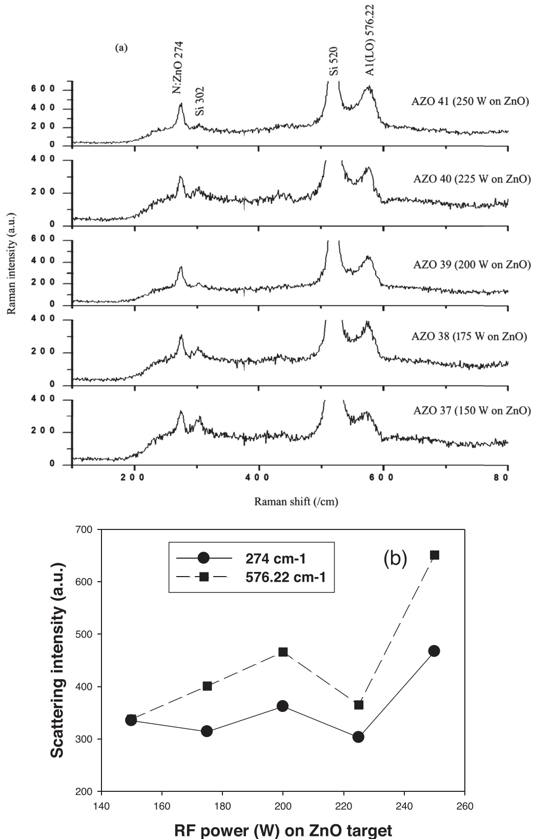
Fig. 8. (a) Raman spectra of AlN: ZnO thin films and (b) modes intensity variation at different RF on Si substrates.
