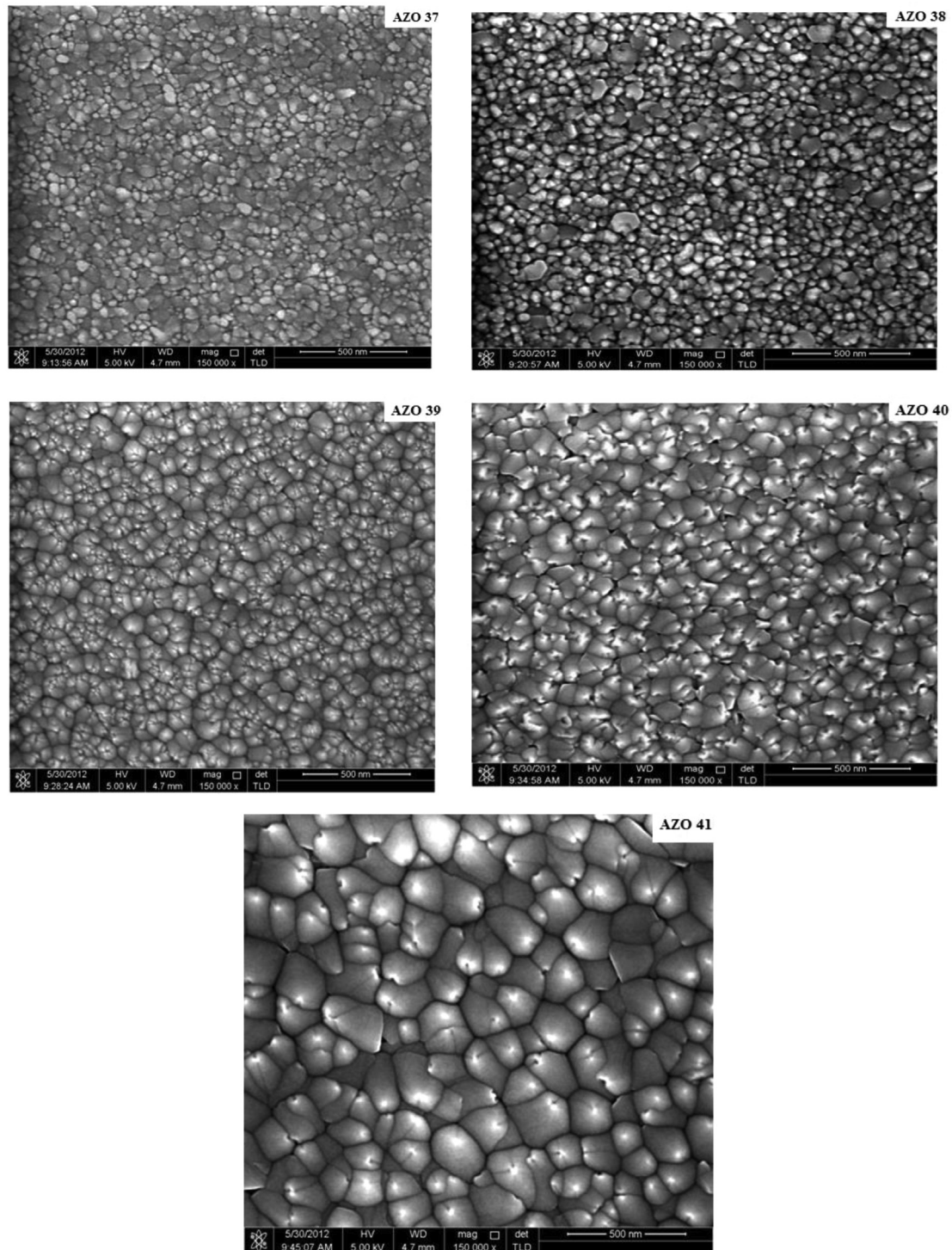
Fig. 3. FE-SEM images of AlN: ZnO thin films at different RF powers on Si substrates.
