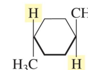
trans -1,4-dimethylcyclohexane
