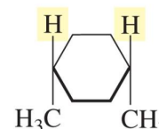
cis -1,4-dimethylcyclohexane
