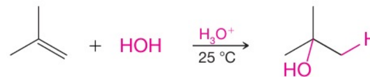
2-Methylpropene (isobutylene)
