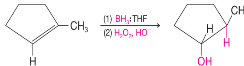
1-Methylcyclopentene
