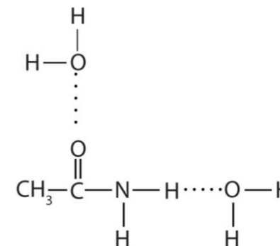
Hydrogen bonding between amide and water molecules
