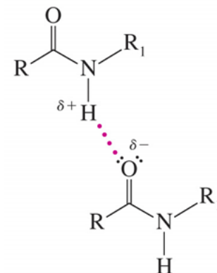
Hydrogen bonding between amide molecules
