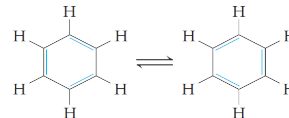
The Kekulé structures for Benzene
