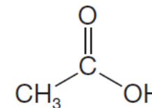
Acetic acid pK_a = 4.75
