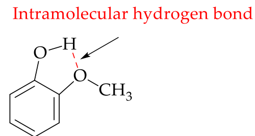
o -Methoxyphenol m.p = 204-206 °C
