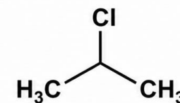
2-Chloropropane
