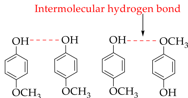
p -Methoxyphenol m.p = 243 °C
