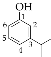
3-Isopropylphenol
