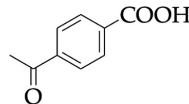
4-Acetylbenzoic acid
