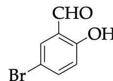
5-Bromo-2-hydroxybenzaldehyde
