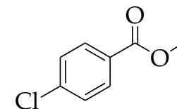
Methyl p-chlorobenzoate
