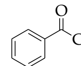
Benzoyl chloride
