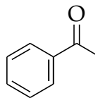
1-Phenylethanone Acetophenone
