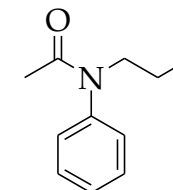
N-Phenyl-N-propylethanamide
