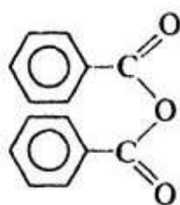
Benzoic anhydride
