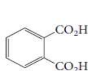
phthalic acid
