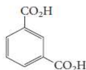
isophthalic acid
