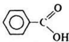
Benzoic acid
