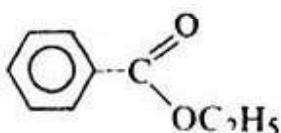
Ethyl benzoate
