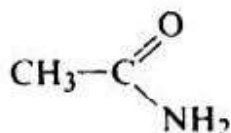
Acetamide Ethanamide
