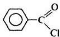
Benzoyl chloride
