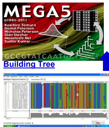
DNA sequence alignment using ClustalX
