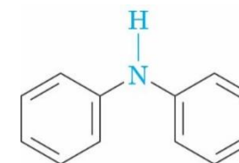
Diphenylamine
