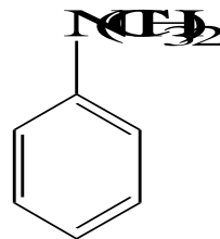
N,N-Dimethylaniline (N,N-Dimethylaniline)
