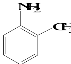
o-Toluidine
