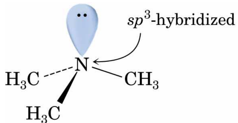
Trimethylamine
