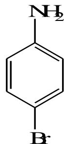
p-Bromaniline (4-Bromobenzenamine)
