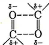
Dipole-dipole attractions among carbonyl compounds
