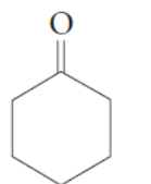
cyclohexanone
