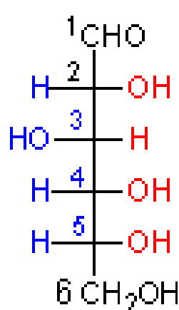
D-glucose
