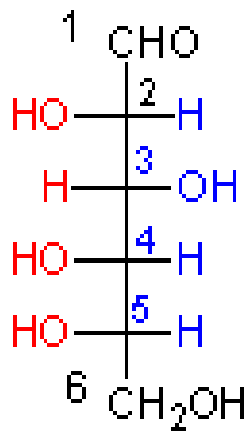
L-glucose
