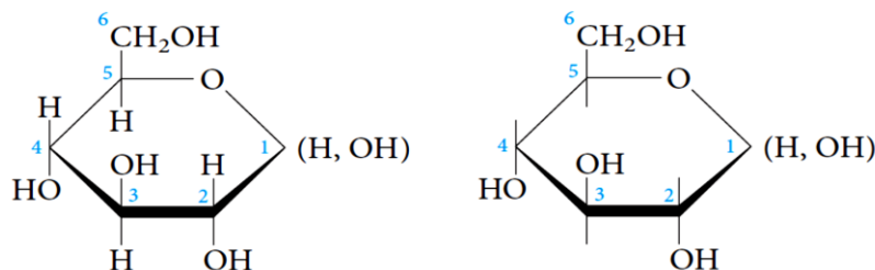
Haworth projection formulas for D-glucose
