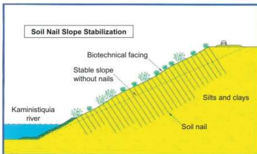
Figure 21.17 Soil nail and root solution for Kaministiquia riverbank slopes.
