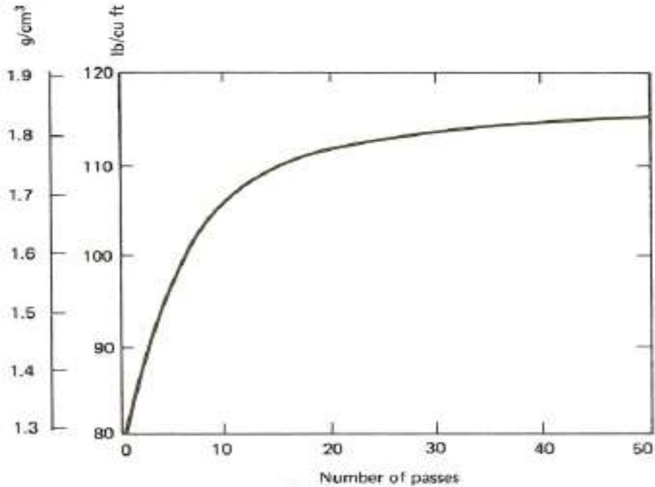
FIGURE 5-12: Typical effect of number of passes.
