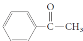
acetophenone (methyl phenyl ketone) 1-phenylethanone
