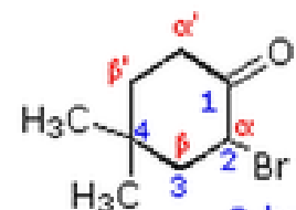
2-bromo-4,4-dimethylcyclohexanone
