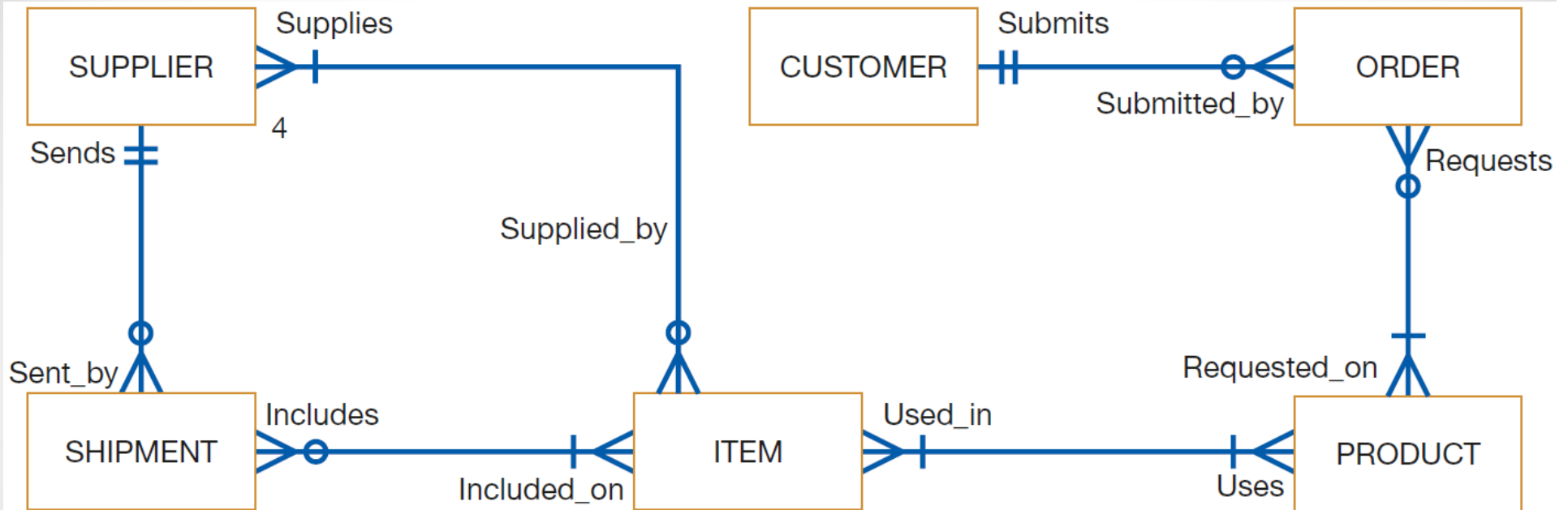
Sample conceptual data model
