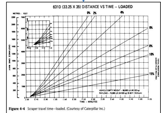
Figure 4-4 Scaper travel time—loaded. (Courtesy of Caterpillar Inc.)
