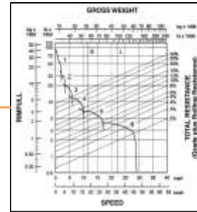
Performance Curve Wheel
