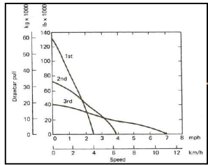
Performance Curve Tractor
