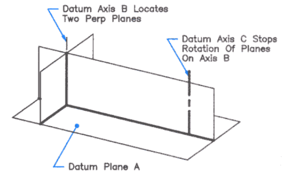
Figure 6-32. A primary datum surface and secondary datum feature of size can be used to establish the datum reference frame with a tertiary datum feature of size used to set the orientation of the datum reference frame.
