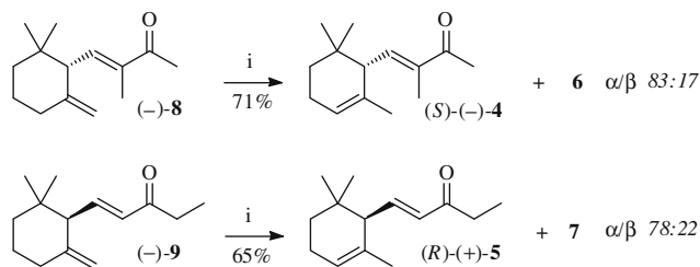
Scheme 4. Chemical correlation of enantioenriched \gamma -iralia isomers 8 and 9 with enantioenriched \alpha -iralia isomers 4 and 5 . Reagent and condition: (i) 85% H 3 PO 4 .
