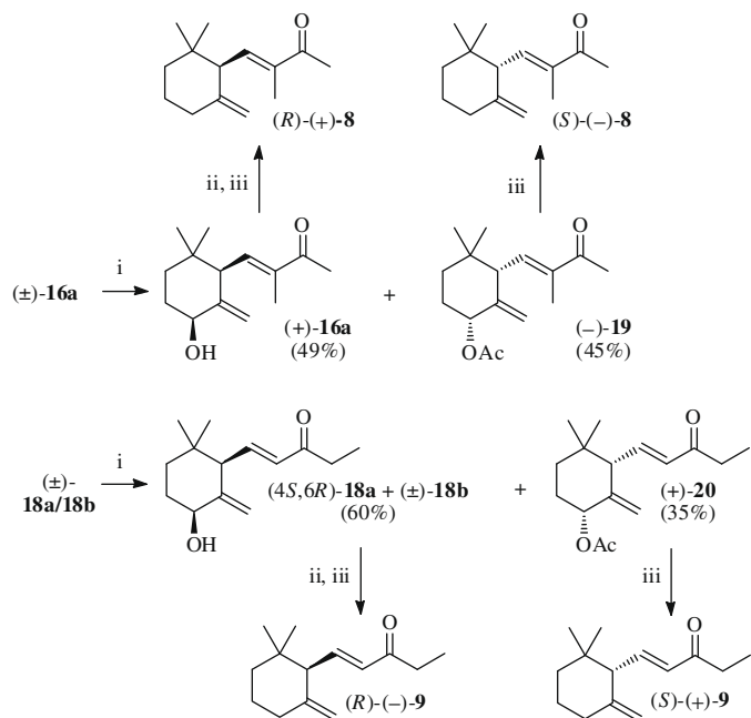
Scheme 3. Preparation of enantioenriched \gamma -iralia isomers 8 and 9 . Reagents and conditions: (i) vinyl acetate, t -BuOMe, lipase PS; (ii) Ac 2 O/Py; (iii) HCOOH, Et 3 N, PPh 3 , PdCl 2 (PPh 3 ) 2 cat., THF, reflux.
