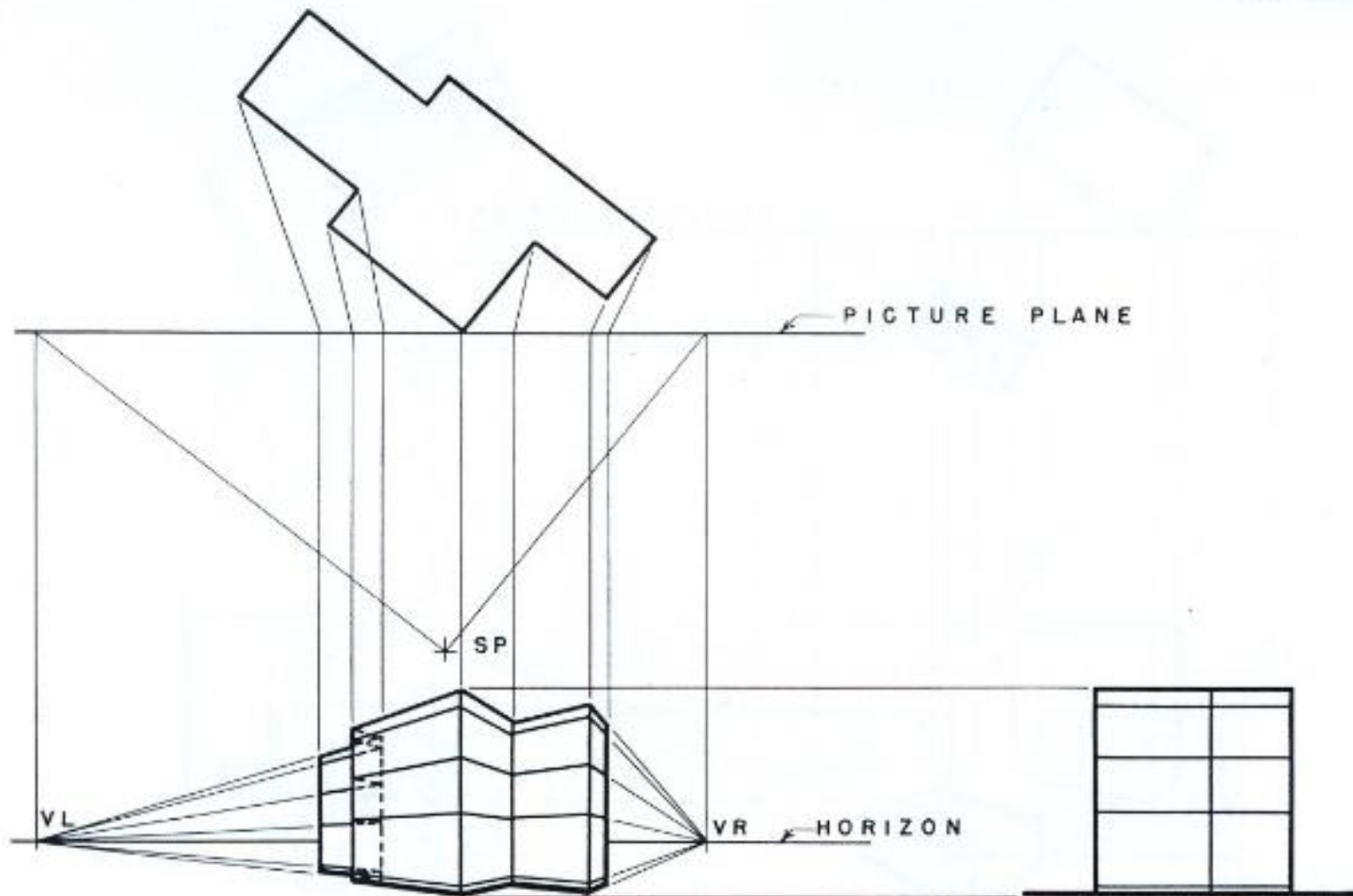
HEIGHTS CARRIED AROUND CORNERS
