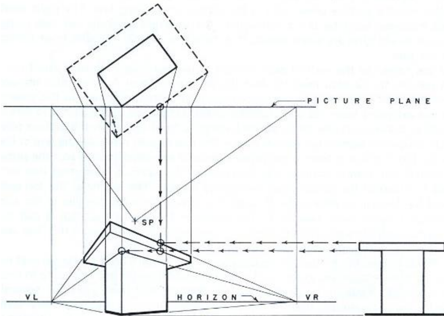
OBJECT EXTENDING THROUGH PICTURE PLANE
