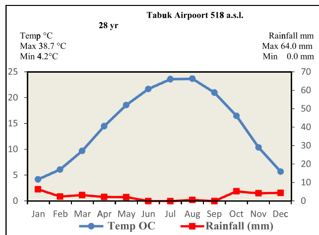
Fig. 2. Tabuk climate diagram, Saudi Arabia (1987–2015).
