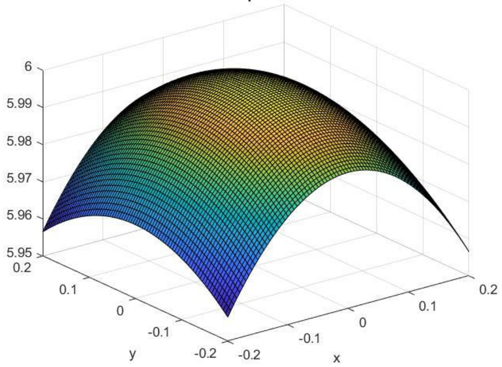
Ellipsoid
