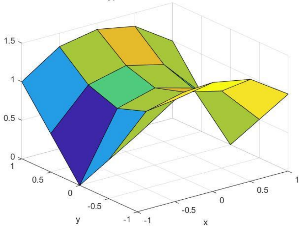
Hyperboloid of one sheet
