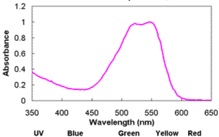
Molecular absorption spectrum
