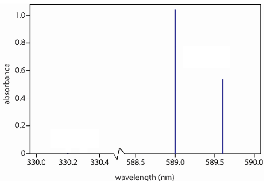
Atomic absorption spectrum
