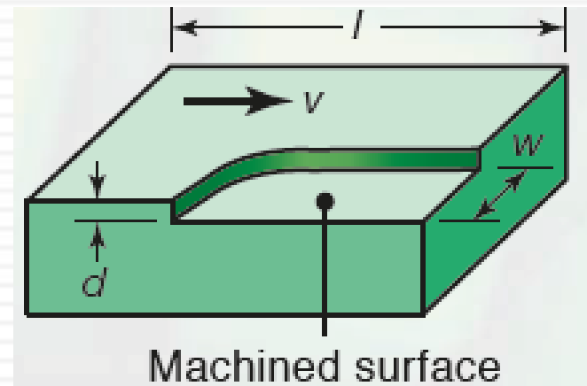
Dimensions in face milling
