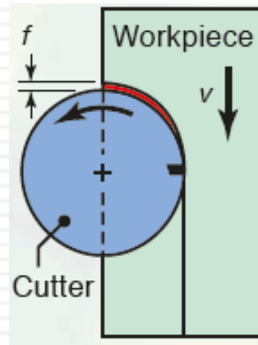
Conventional milling
