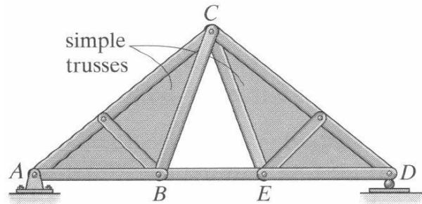
compound truss
