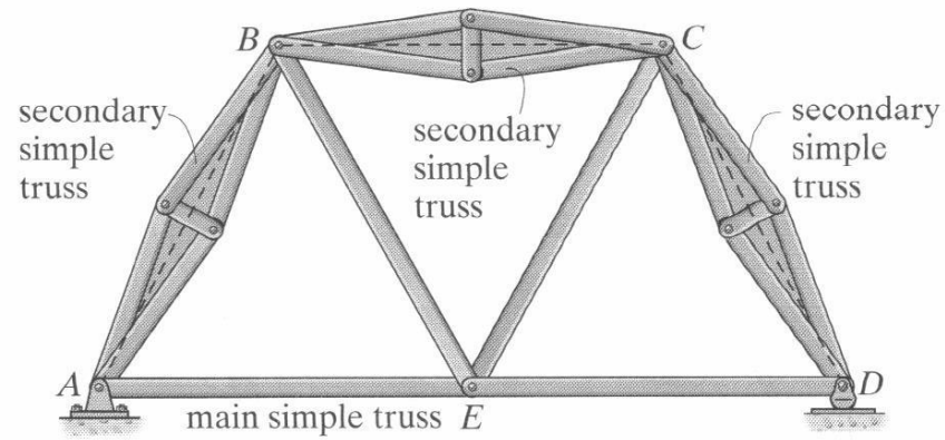
compound truss
