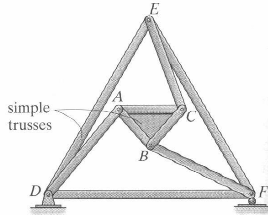
compound truss
