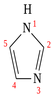
Imidazole
