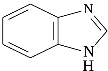
Benzo[d]-1,3-diazole
