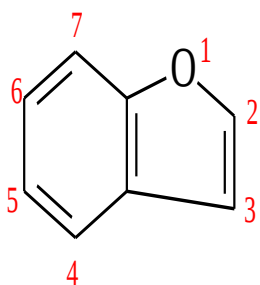
Benzo[b]furan
