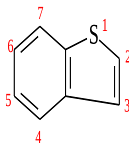
Benzo[b]thiophene
