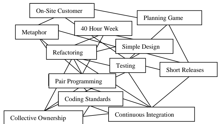
Figure 2. Dependencies between the 12 practices.
