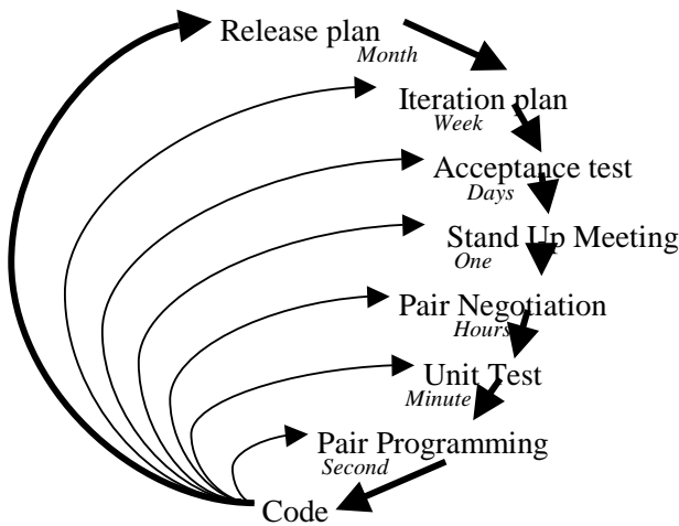
Figure 3. Planning/feedback loops in XP.
