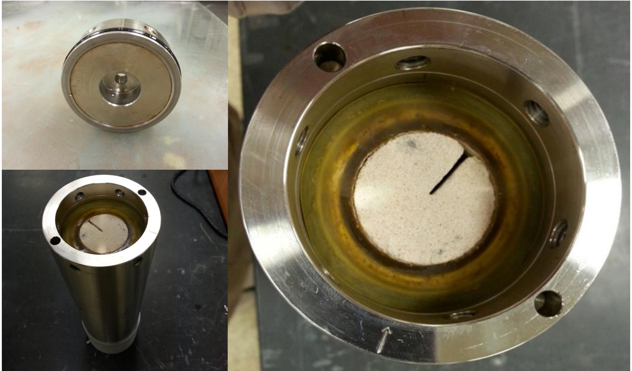
Modification of the API HT-HP Filtration Cell to Accommodate the Man-made Fractured Core
