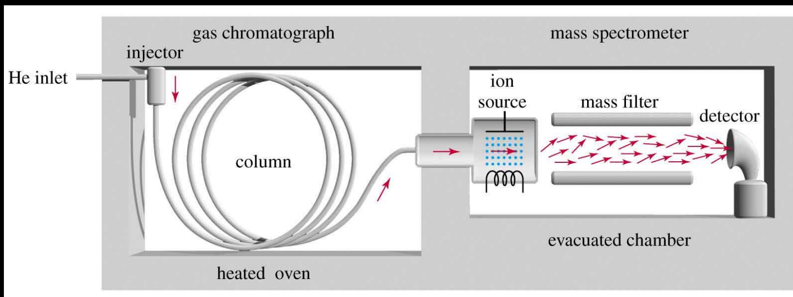
Figure 1 : GC – MS Combination
