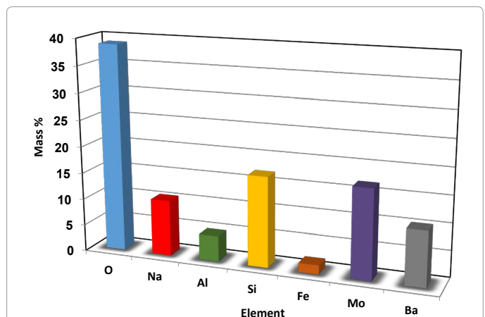
Figure 19: Chemical Composition of the filter cake Using SEM, sample 1 (0.0 gm XC – Polymer).
